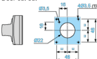
Door cut-out
